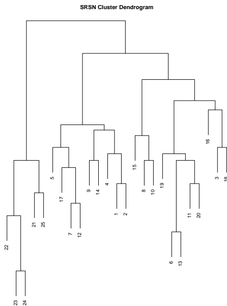
(a) Dendrogram for SRSN, clustered by Euclidean distance. We observe three different clusters of nodes.
