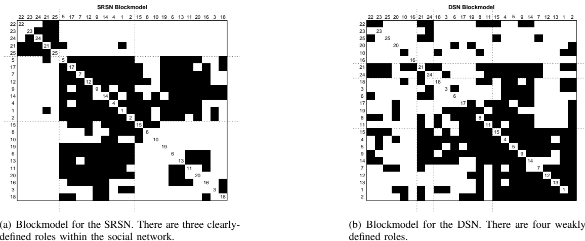
Fig. 3. Blockmodels of role equivalence for the SRSN and DSN. Dotted lines indicate role divisions.
